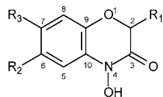
R_1=OH ; R_2=R_3=H : 2,4-Dihydroxy-(2 H )-1,4-benzoxazin-3(4 H )-one (DIBOA) R_1=OH ; R_2=H ; R_3=OCH_3 : 2,4-Dihydroxy-7-methoxy-(2 H )-1,4-benzoxazin-3(4 H )-one (DIMBOA) R_1=R_2=R_3=H : 4-Hydroxy-(2 H )-1,4-benzoxazin-3(4 H )-one (D-DIBOA) R_1=H ; R_2=OCH_3 ; R_3=H : 4-Hydroxy-6-methoxy-(2 H )-1,4-benzoxazin-3(4 H )-one (6-MeO-D-DIBOA)
